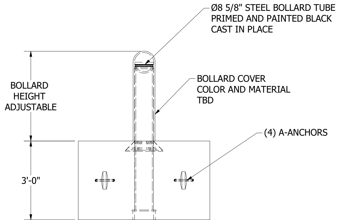
PROFILE VIEW
